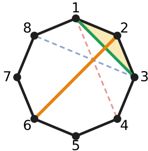
slot \{X_{2,\ell}, \dots, X_{k,\ell}\}
